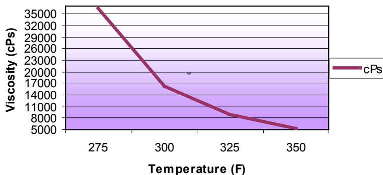
Typical Viscosity Curve
